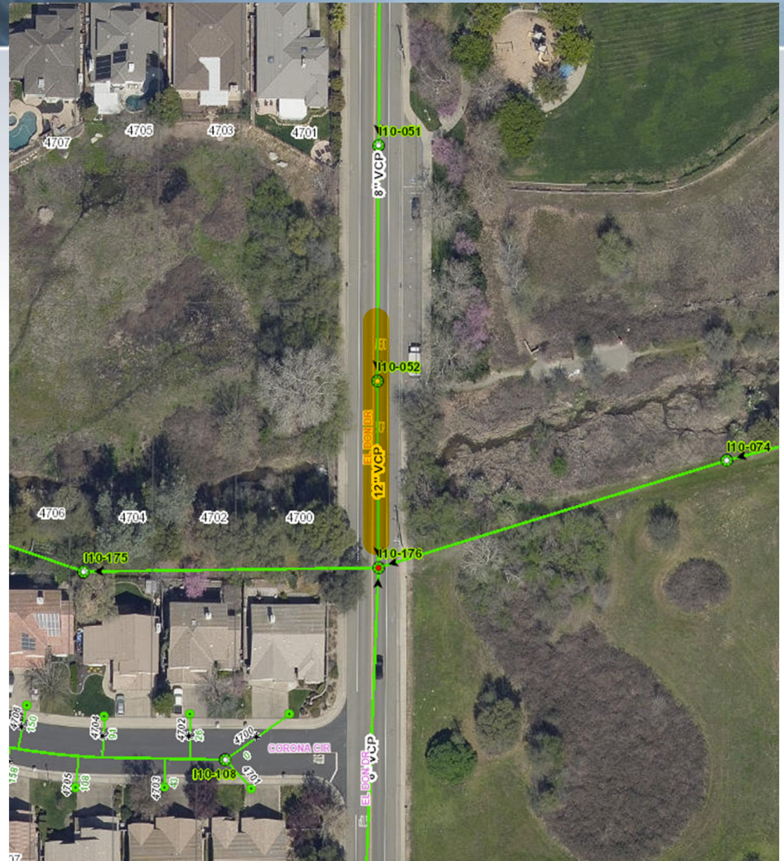
Limits of sewer replacement (highlighted in yellow).
